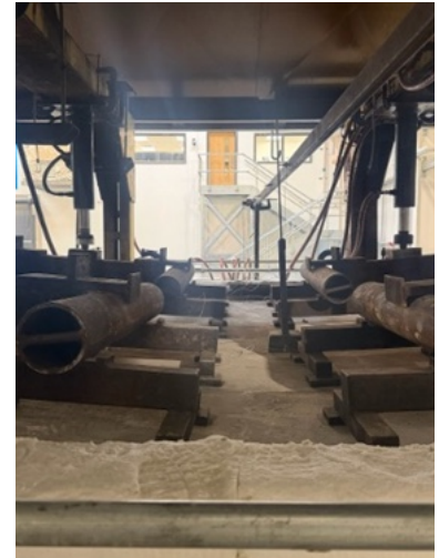
Apply 5.5 Kpa on the Test Specimen
