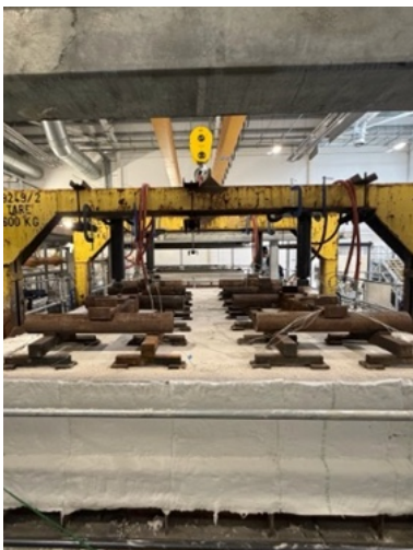
Slab Ready for the Fire Test
