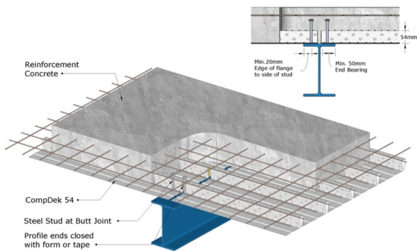
CompDek 54 - Butt Joint
