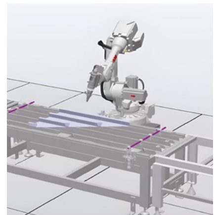
Robotic Cutter
