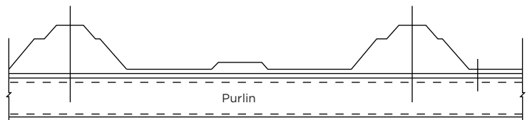
Crest fixing for roofs or walls.
