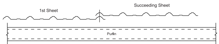
Pan fixing for walls only.
