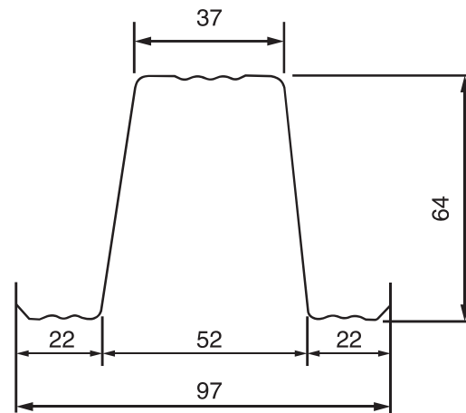
Measurement : 64mm x 37mm x 22mm
