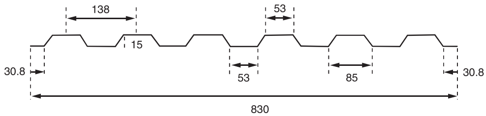
Cover Width of SundeK 830: 830mm
