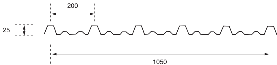
Cover Width of SundeK 1050: 1050mm
