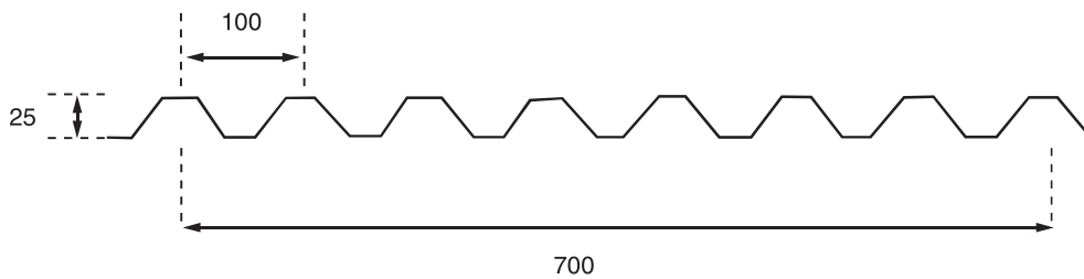
Cover Width of Swandek : 700mm
