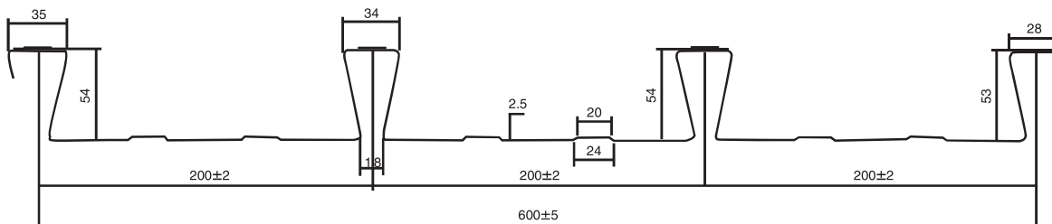
Cover Width of Compdek : 600mm
