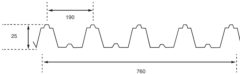
Cover Width of SundeK 760: 760mm
