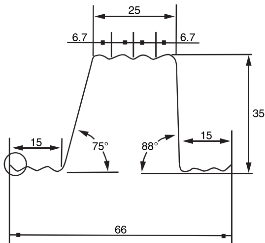
Measurement : 35mm x 25mm x 15mm
